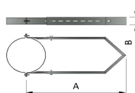
HIS5 SOPORTE MURAL DE ESQUINA CORNER WALL SUPPORT
