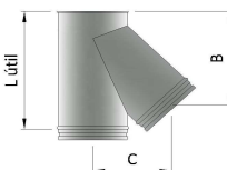
BITS TE 135° ESTANCA TEE 135° TIGHTNESS
