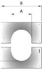
HIPE PLACA EMBELLECEDORA 0° A 30° FINISHING PLATE 0° TO 30°
