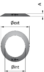
HILM COLLARÍN ANTILLUVIA CORTO SHORT STORM COLLAR
