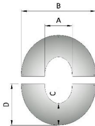
HIPW PLACA EMBELLECEDORA REDONDA 150 45° ROUND FINISHING PLATE 150 45°
